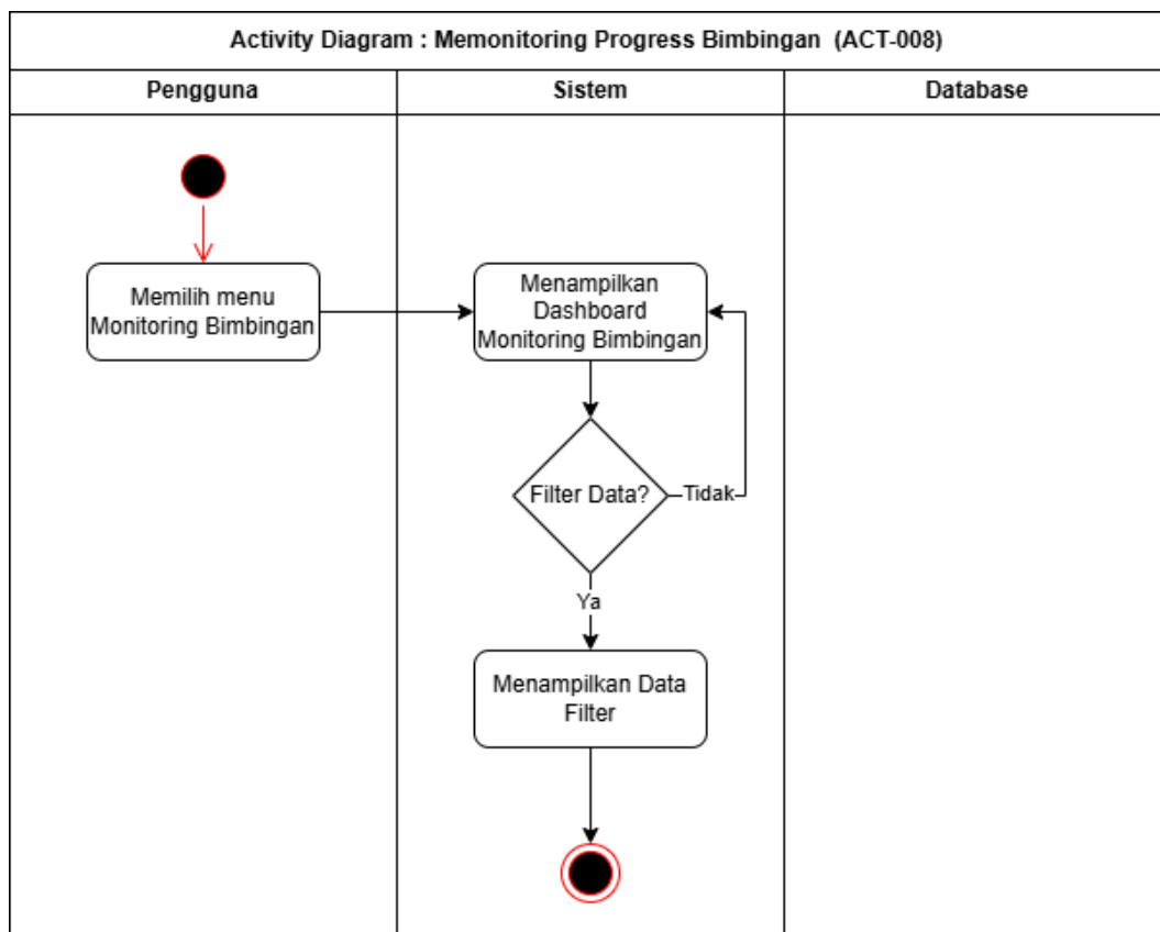
Gambar 3. 9 Activity Diagram Memonitoring Progres Bimbingan.
